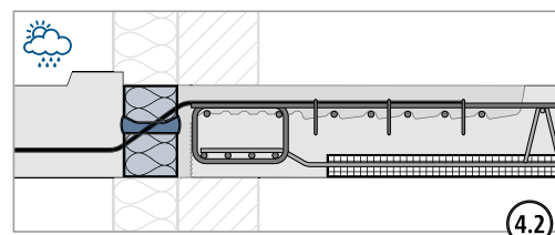
Isokorb® XT/T type Q-E, Q-T
